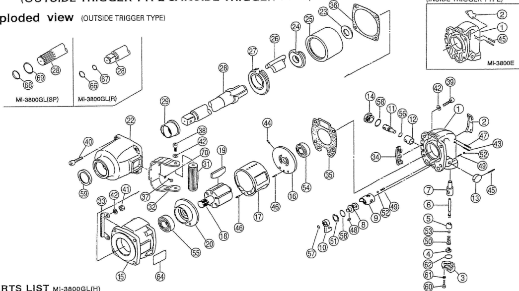
PARTS LIST MI-3800GL(H)
